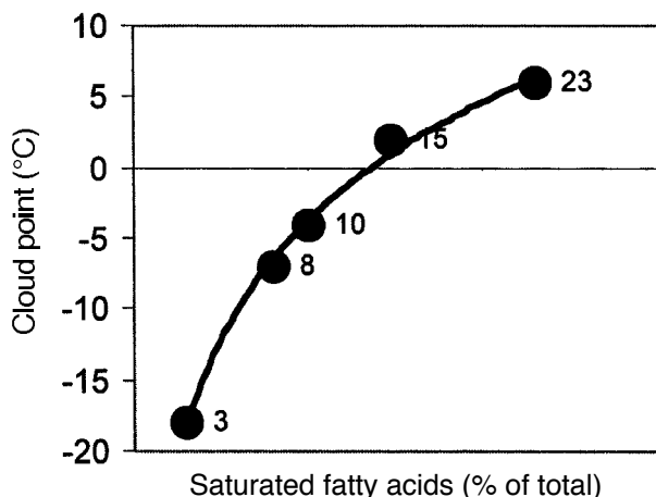
Fig. 1. Soy biodiesel cloud point and saturated fat content. Data for samples with 8, 15, and 23% (hydrogenated soy) saturated fat are from References 7, 8, and 9, respectively.
