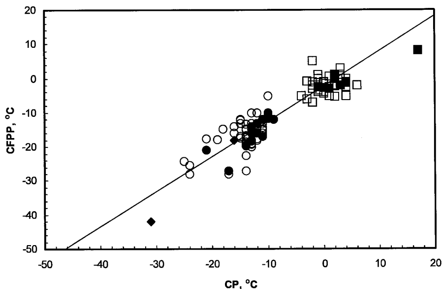
Fig. 3. Cold filter plugging point (CFPP) vs. cloud point (CP) for biodiesel/petrodiesel blends. Legend: ◆ = petrodiesel (B0); ■ = neat biodiesel (B100); □ = B100 + CFI; ● = blends; ○ = blends + CFI. Biodiesel = fatty acid methyl esters; CFI = cold flow improver. Regression line: CFPP = 1.0276[CP] - 2.2 ( R^2 = 0.82 , \sigma_y = 3.5 ).
