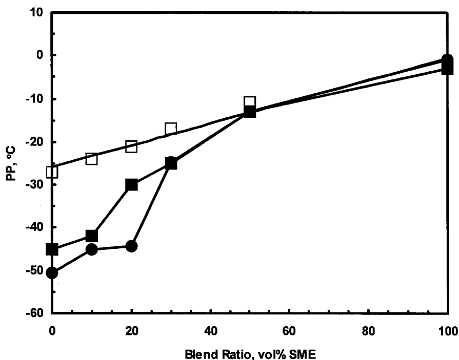
Fig. 2. Pour point (PP) vs. blend ratio (vol%) of soybean oil fatty acid methyl esters (SME) for blends with No. 1 (D-1) and No. 2 (D-2) diesel fuels and JP-8 jet fuel. Legend: \square = D-2 blends; \blacksquare = D-1 blends; \bullet = JP-8 blends. Line through D-2 blend data: PP = 0.2519[\text{blend ratio}] - 25.8 ( R^2 = 0.96 , \sigma_y = 1.6 ).
