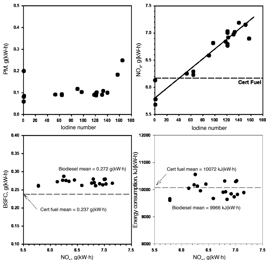
Fig. 3. Effect of biodiesel iodine number on emissions and fuel economy. Data for B100 fuels tested in a 1991 Detroit Diesel Corporation (DDC) Series 60 engine via the heavy-duty transient test. NO x , oxides of nitrogen. Source: Reference 16.
